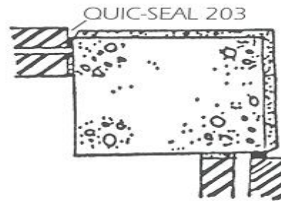
Plan: Brick To Column Detail
