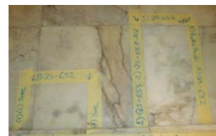
Treatment of rust stains in marble using QUICSEAL 657 Q-Oxidant and QUICSEAL Poultice Powder.
