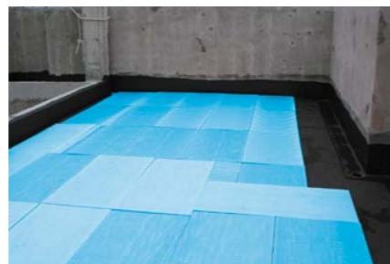
QUICSEAL 102 concealed PU waterproofing with QUICSEAL 704 extruded polystyrene insulation system.
